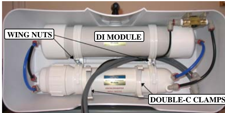
Figure 5. Position of Double-C clamps and wing nuts.
