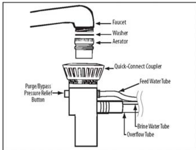
Figure 1. Quick-Connect Faucet Coupler Assembly
