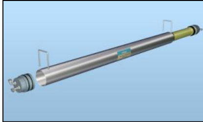
Figure 20: a) remove the connector from one end b) Drag the RO Module out of its casing through the other end
