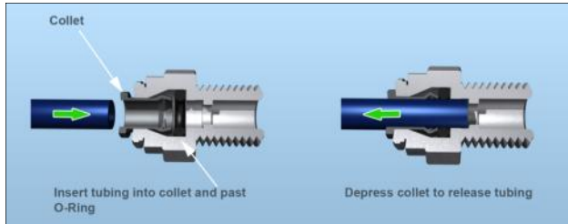
Figure 18: Speedfit Push-in Fittings
