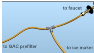
Figure 12. Connect the Ice Maker as shown (color of tubing is for illustrative purposes)
