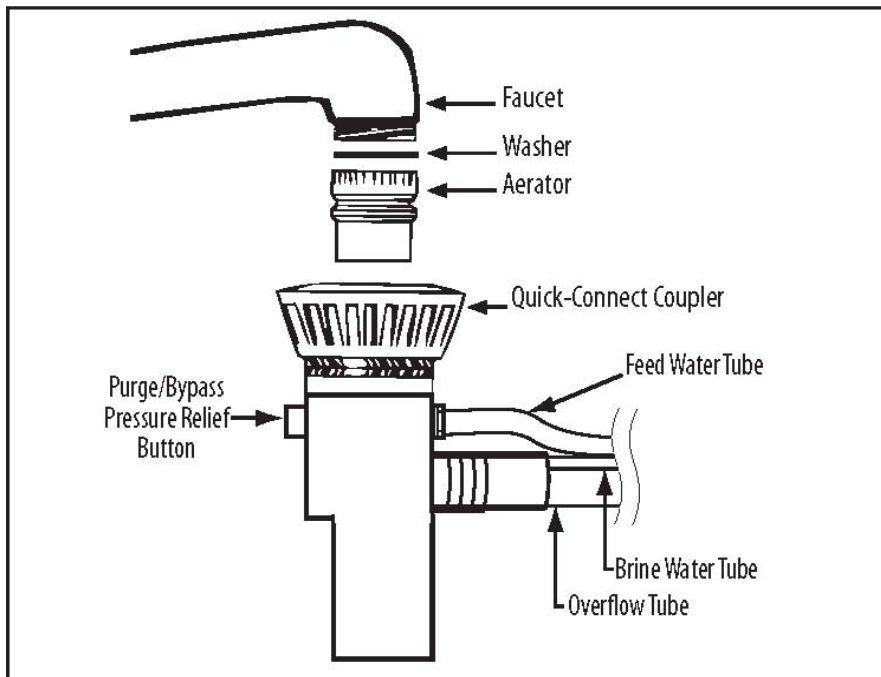
Figure 1. Quick-Connect Faucet Coupler Assembly
