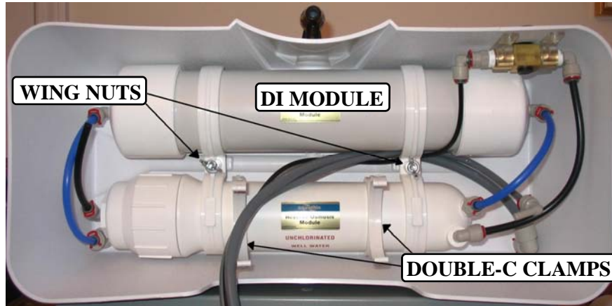
Figure 5. Position of Double-C clamps and wing nuts.
